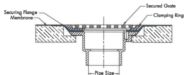
Typical Installation
